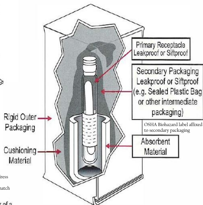
Cross Section of Closed Package
